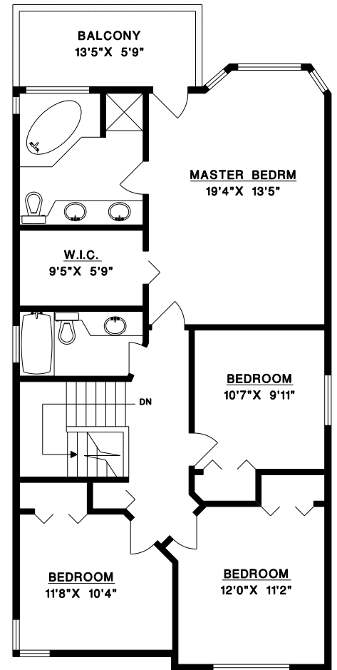
UPPER FLOOR
