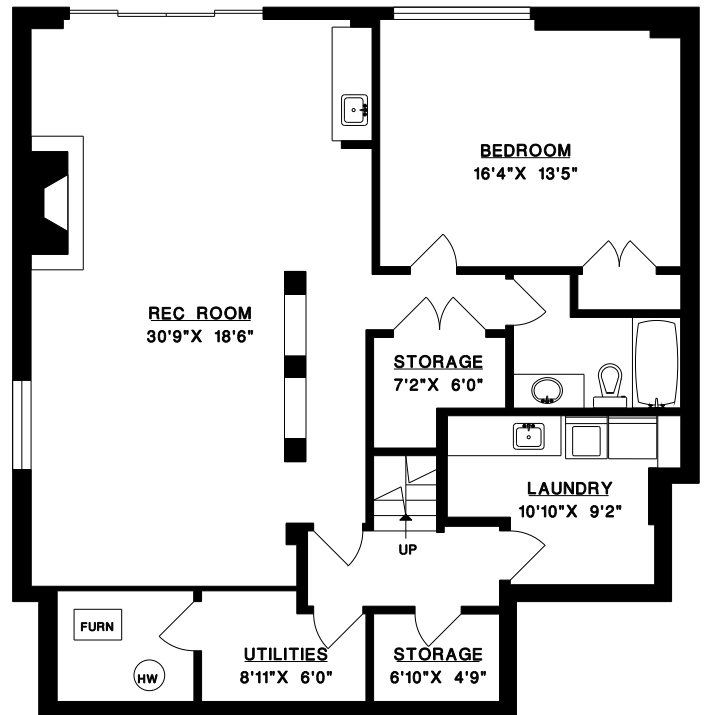
LOWER FLOOR
