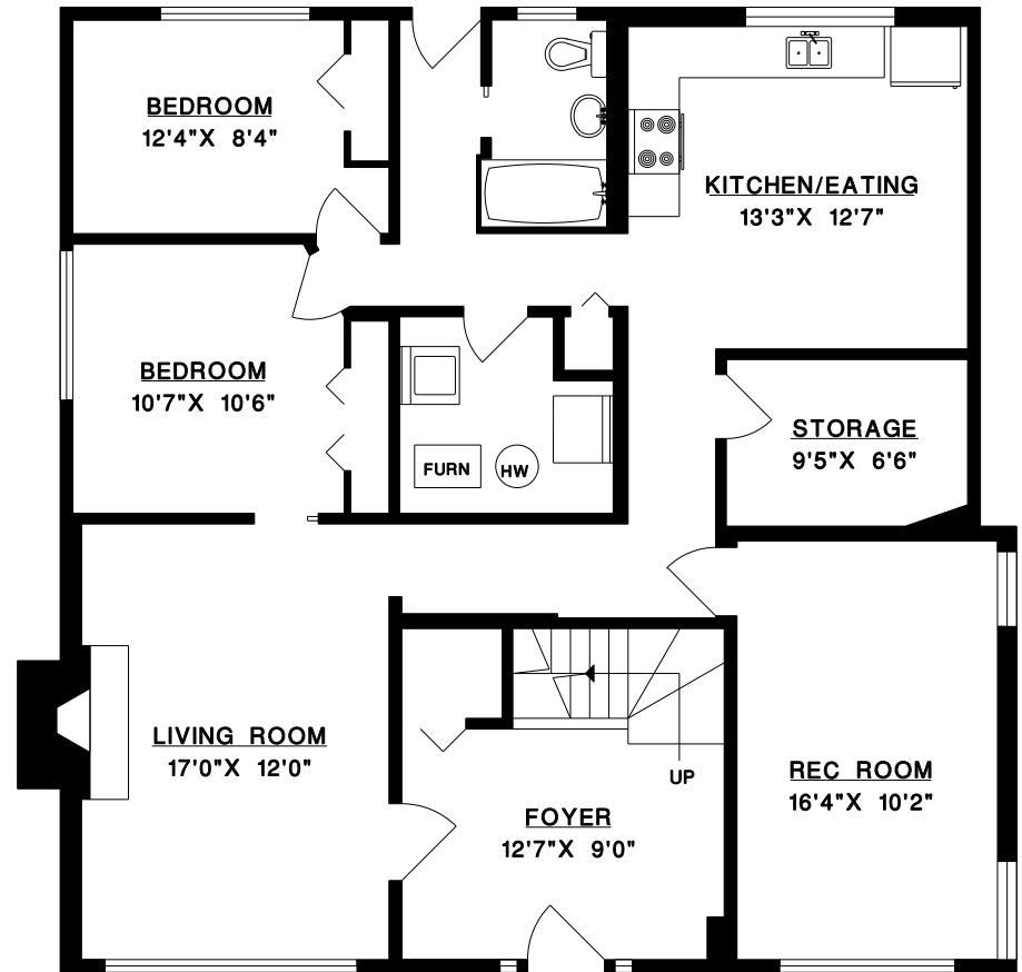
LOWER FLOOR
